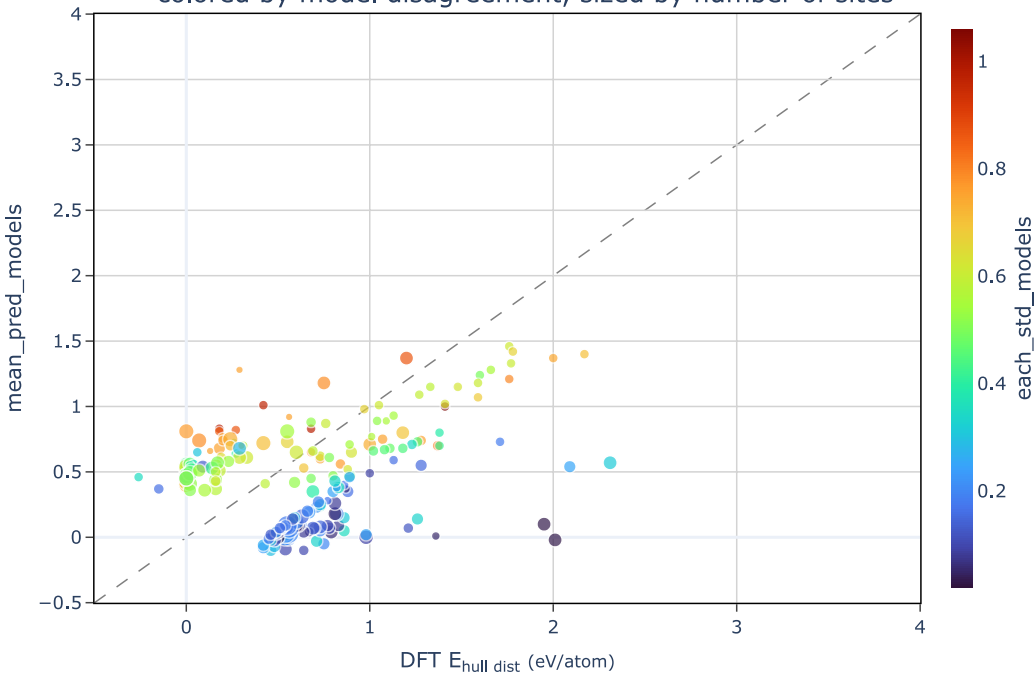
200 oxides with largest hull distance errors colored by model disagreement, sized by number of sites
