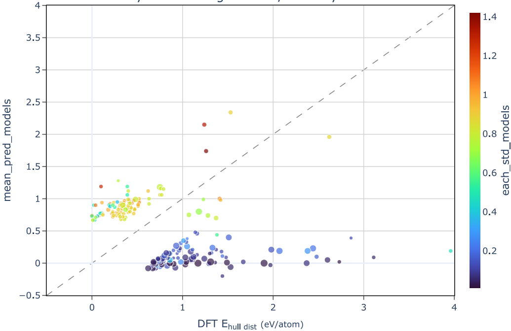
200 pnictides with largest hull distance errors colored by model disagreement, sized by number of sites
