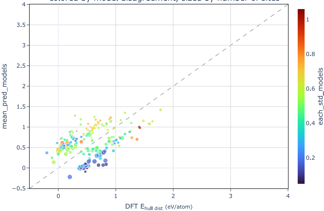
200 sulfides with largest hull distance errors colored by model disagreement, sized by number of sites
