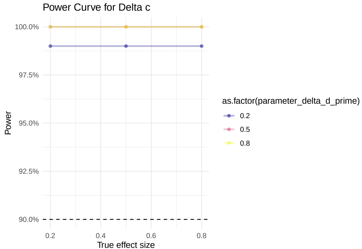
Figure 4. Results of sensitivity analysis for Delta c. The plot shows the power curve, i.e. the share of statistically significant effects across 100 simulated meta-analyses for each pair of values of c (x-axis) and d' (color legend).
