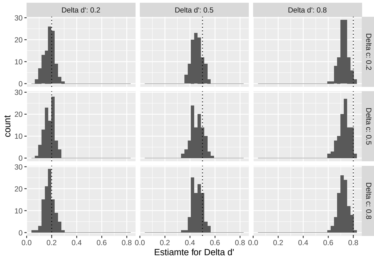
Figure 5. Distributions of Delta d' across simulated meta-analyses. The plot shows the distribution of meta-analytic estimates, for each combination of Delta d' and Delta c values.
