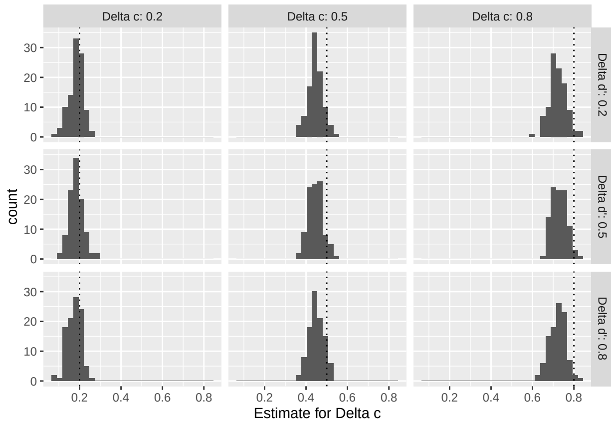
Figure 6. Distributions of Delta c across simulated meta-analyses. The plot shows the distribution of meta-analytic estimates, for each combination of Delta c and Delta d' values.
