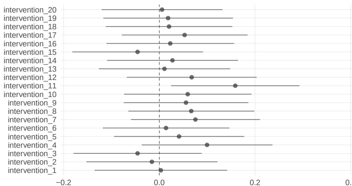
Interaction estimate (per unit increase in moderator)
