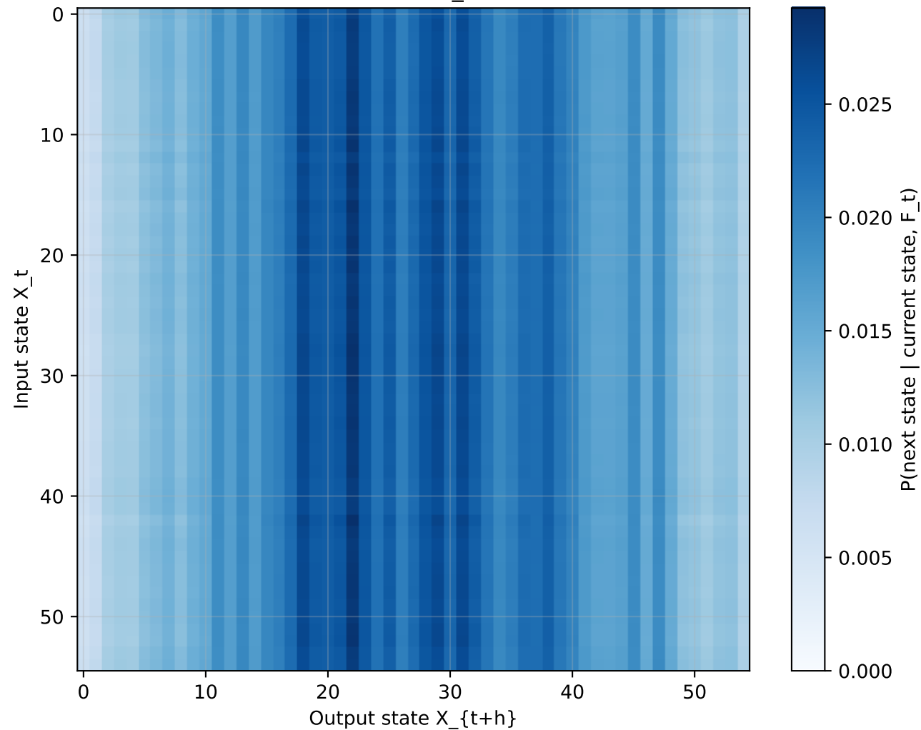
A_t Transition Matrix — t1954 (model: state_cond)
