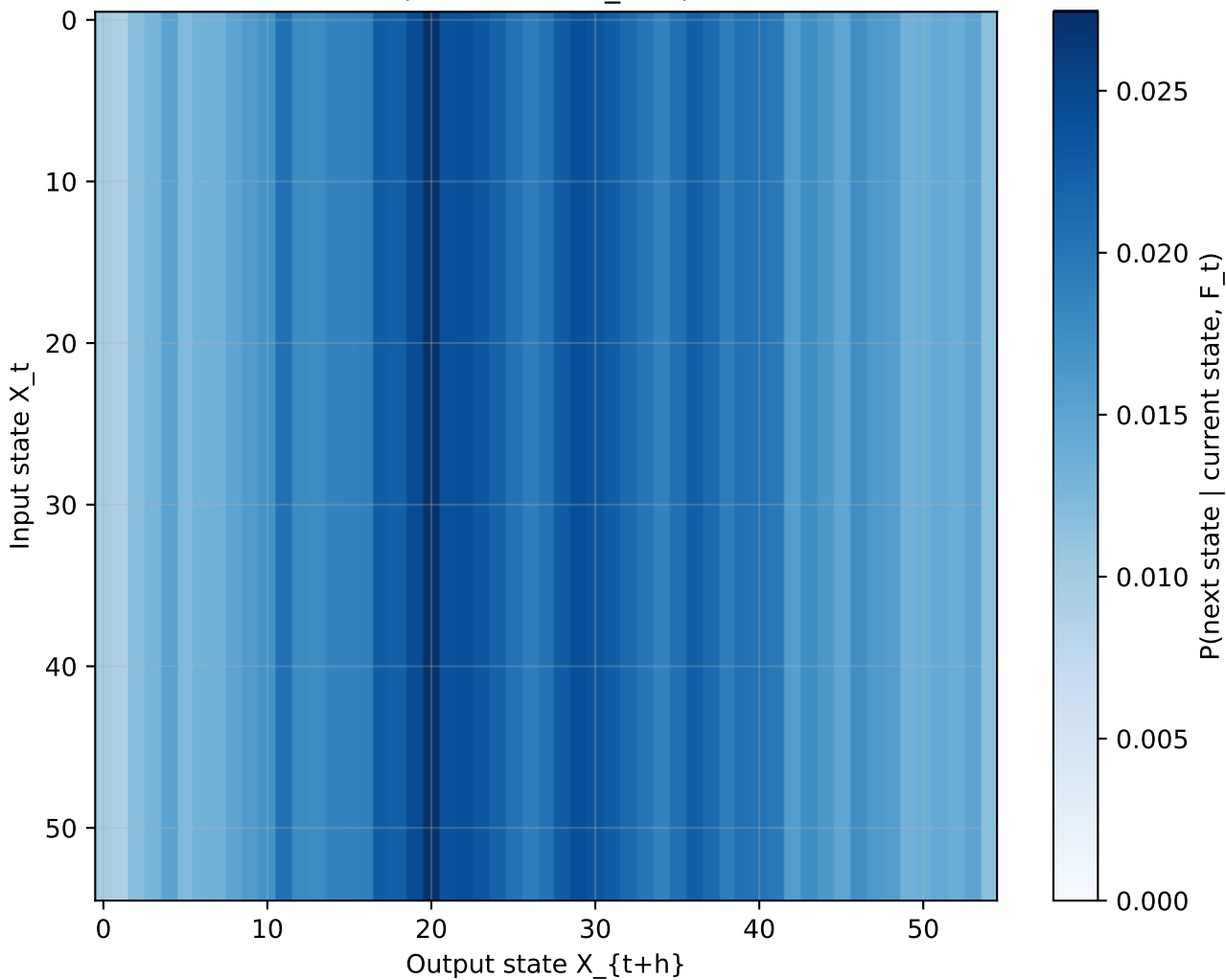
A_t Transition Matrix — t126 (model: state_free)
