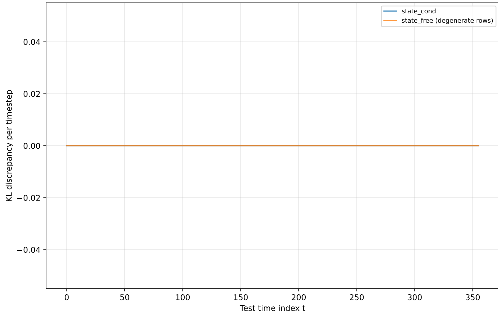
Time-Resolved CK KL Discrepancy (h=1) — Test Period
