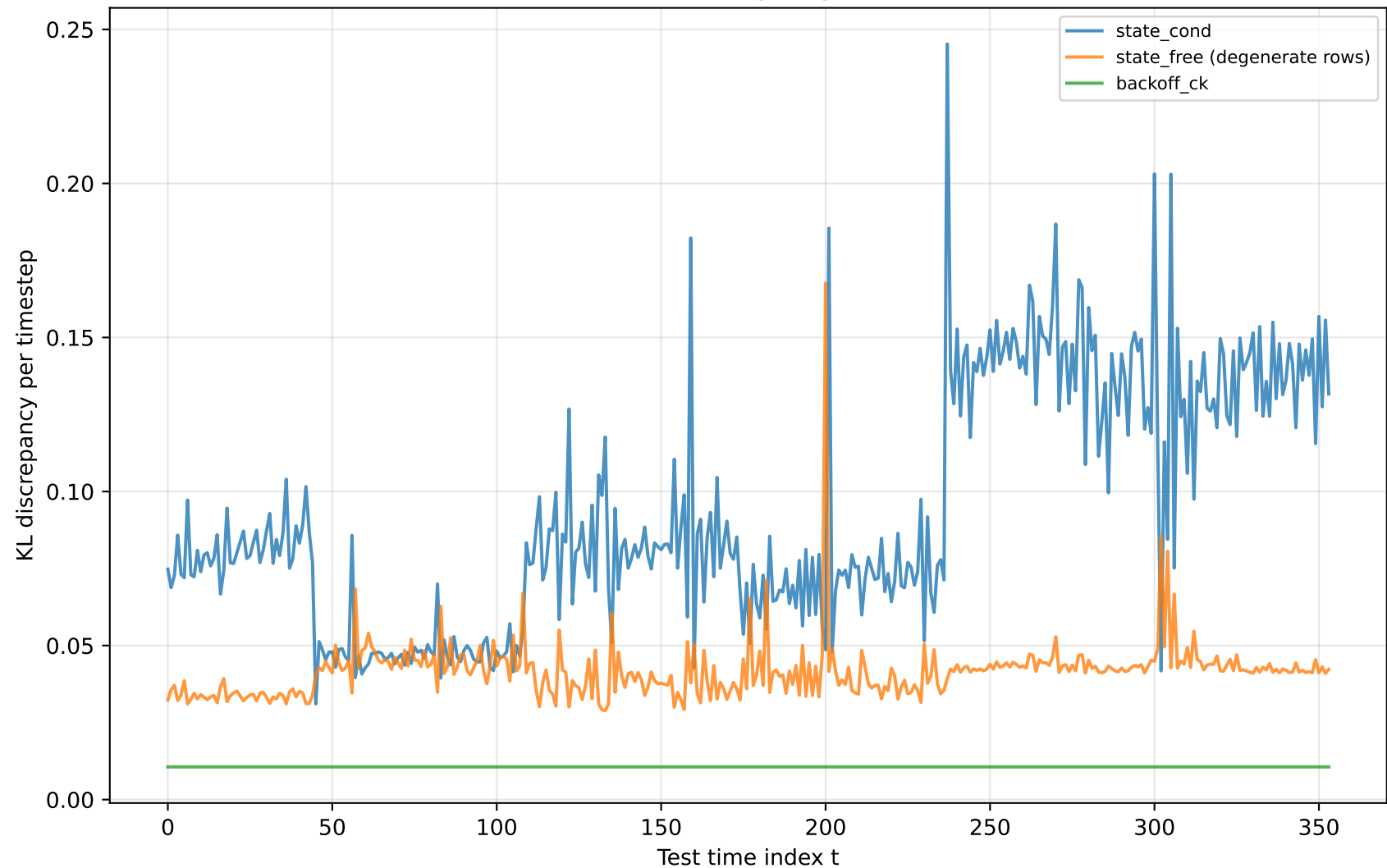
Time-Resolved CK KL Discrepancy (h=2) — Test Period
