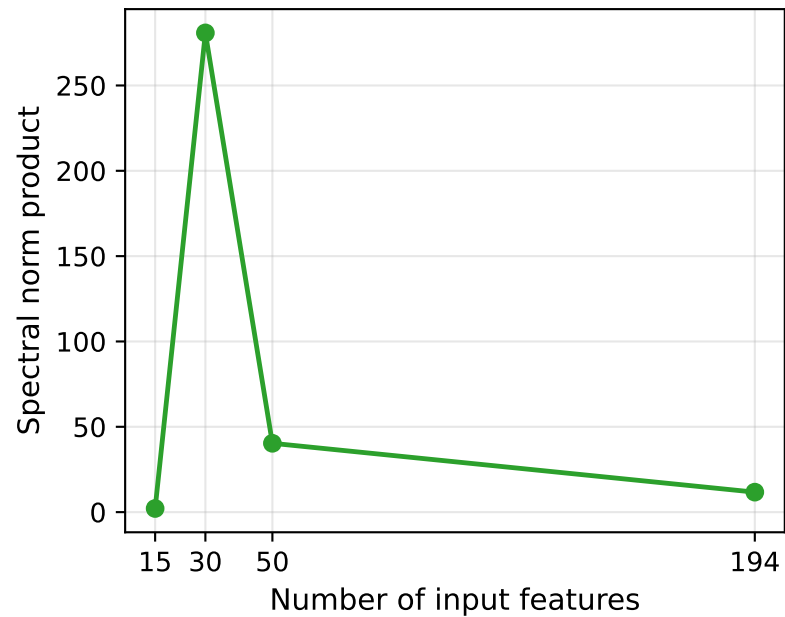
Spectral Norm Product vs Feature Dim
