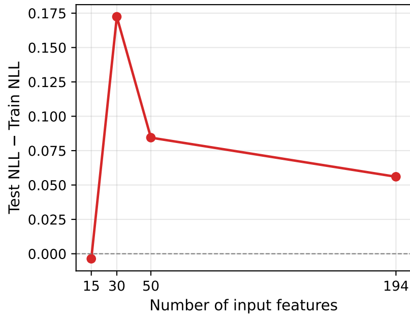
Generalization Gap vs Feature Dim
