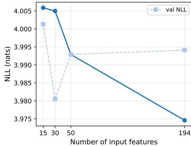
Test NLL vs Feature Dim
