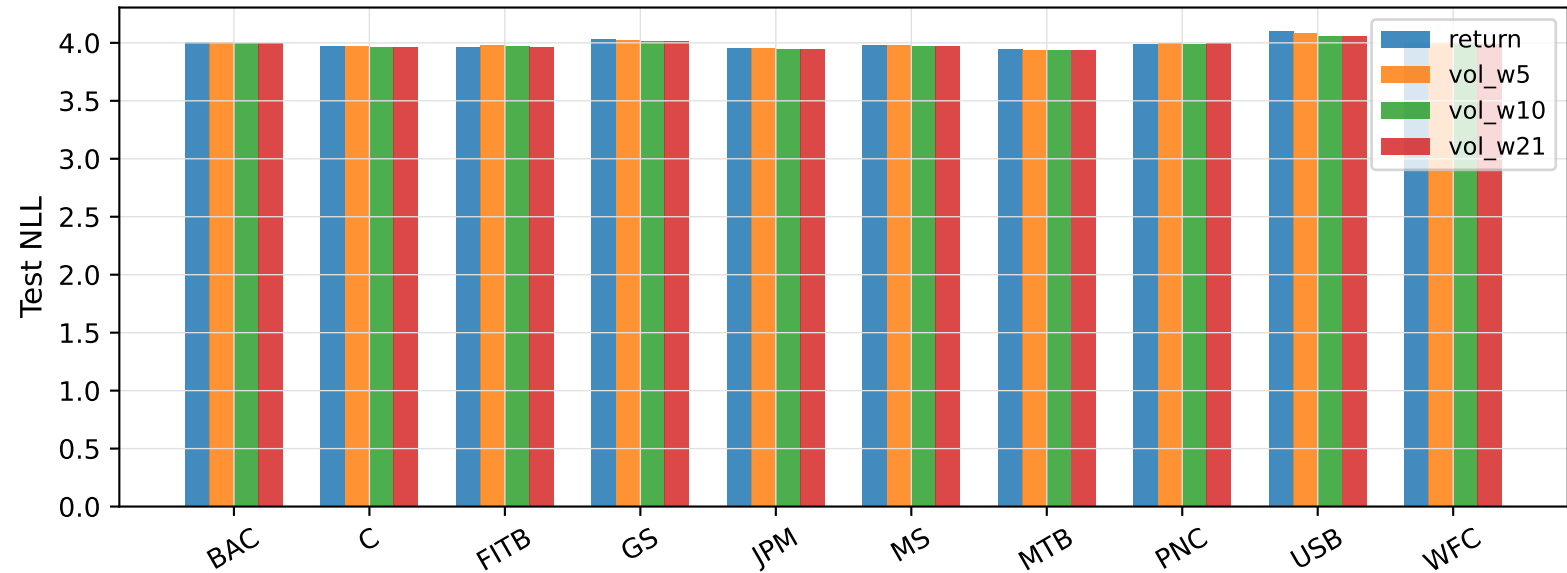
Vol-state vs Return-state (h=1, N=55)
