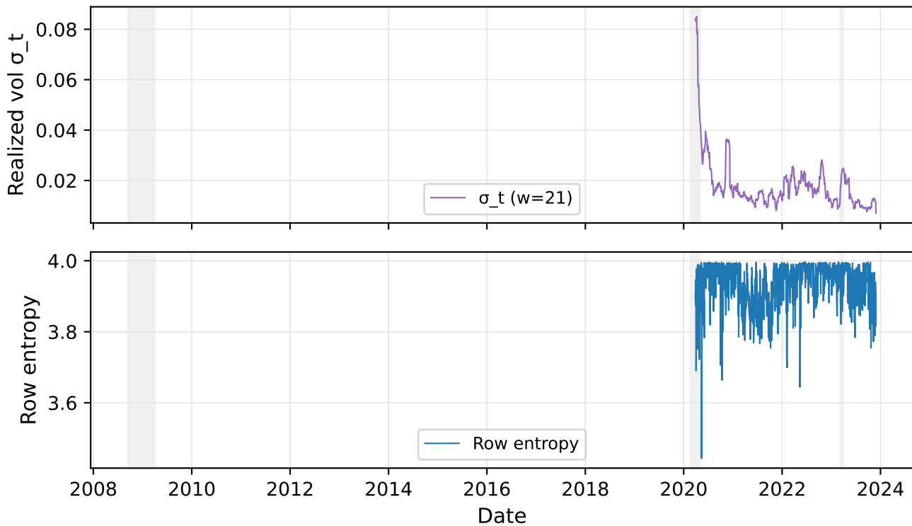
JPM — vol state vs operator row entropy (h=1, N=55)
