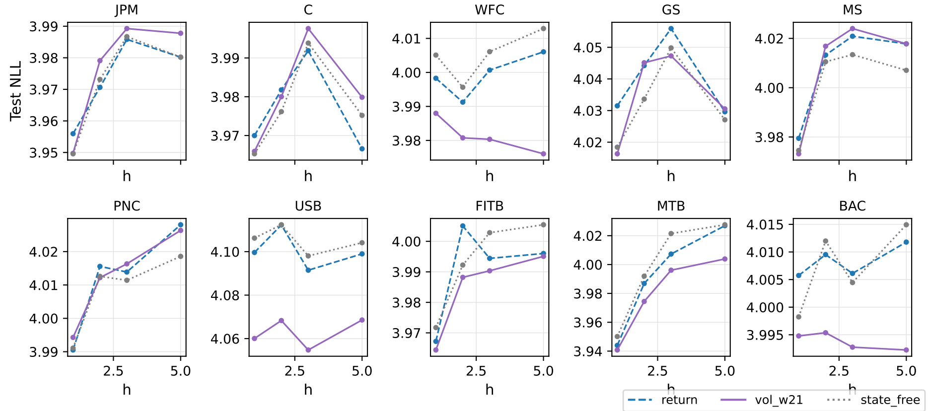
NLL vs horizon: vol-state vs return-state (N=55)
