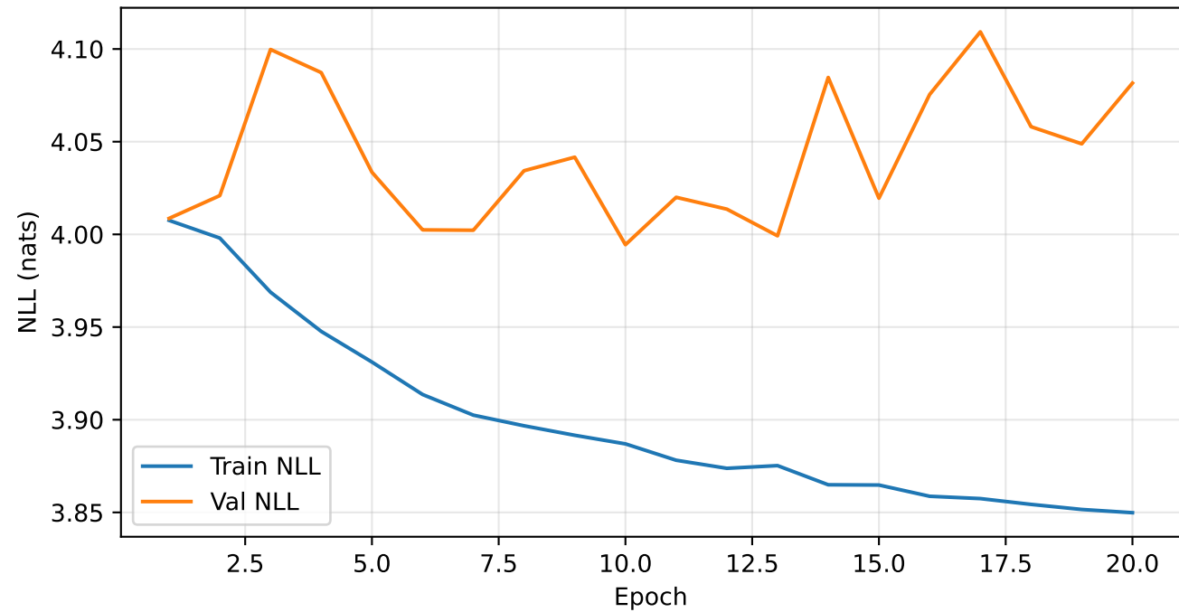
Train vs Val NLL per Epoch
