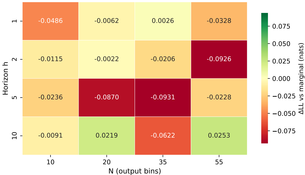
state_cond: \Delta log-likelihood vs marginal (positive = better than marginal; rows = horizon h, cols = N)
