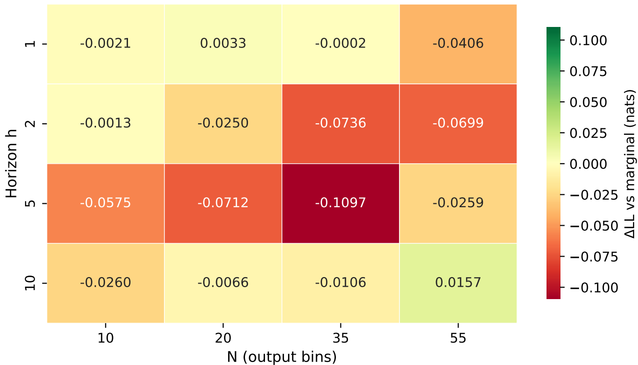
state_free: \Delta log-likelihood vs marginal (positive = better than marginal; rows = horizon h, cols = N)
