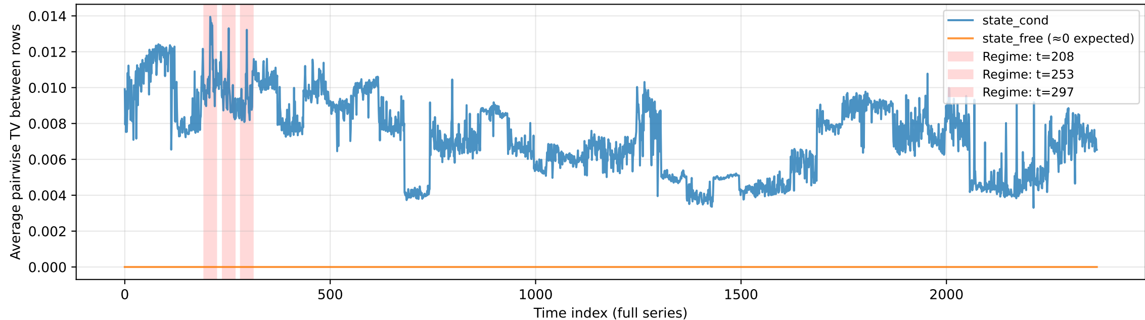
Row Heterogeneity over Time (avg pairwise TV; higher = stronger state dependence)
