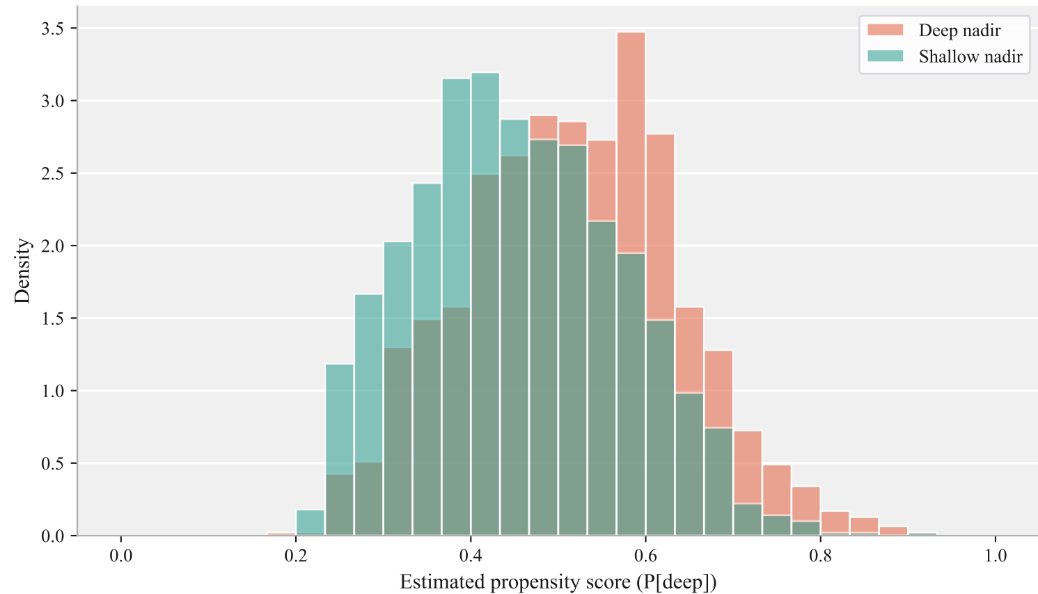
Propensity score overlap
