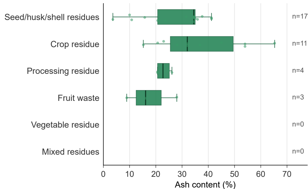
C Ash content (n = 35 treatments)
