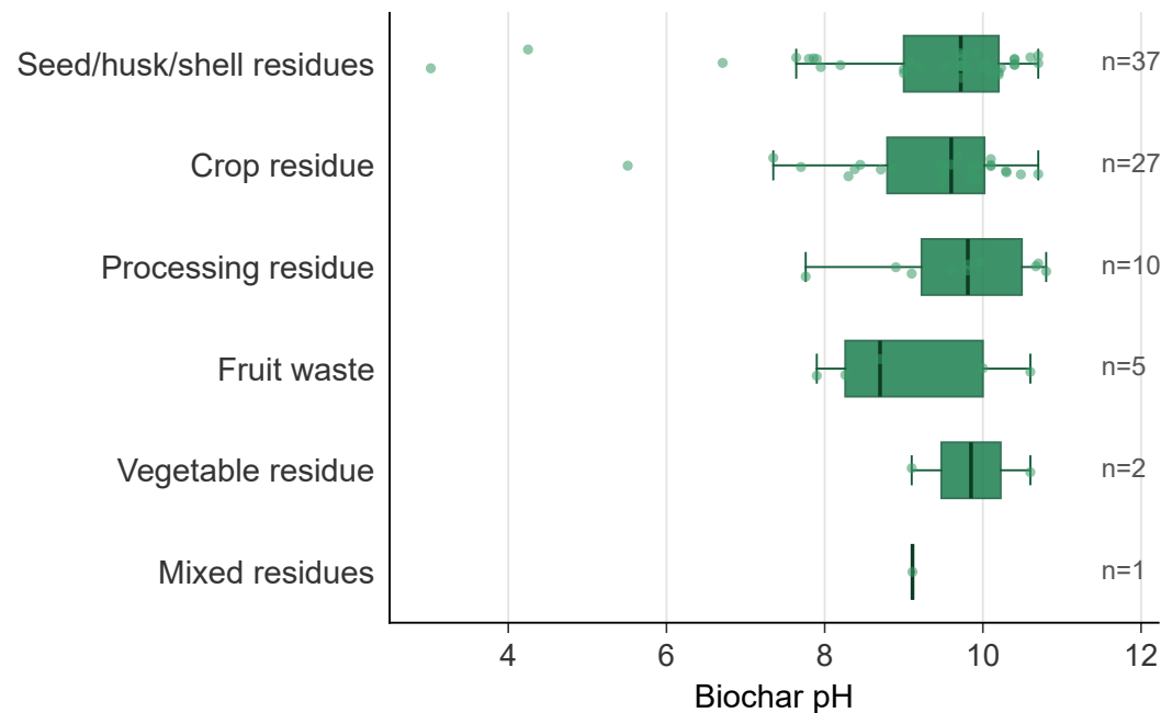
A Biochar pH (n = 82 treatments)
