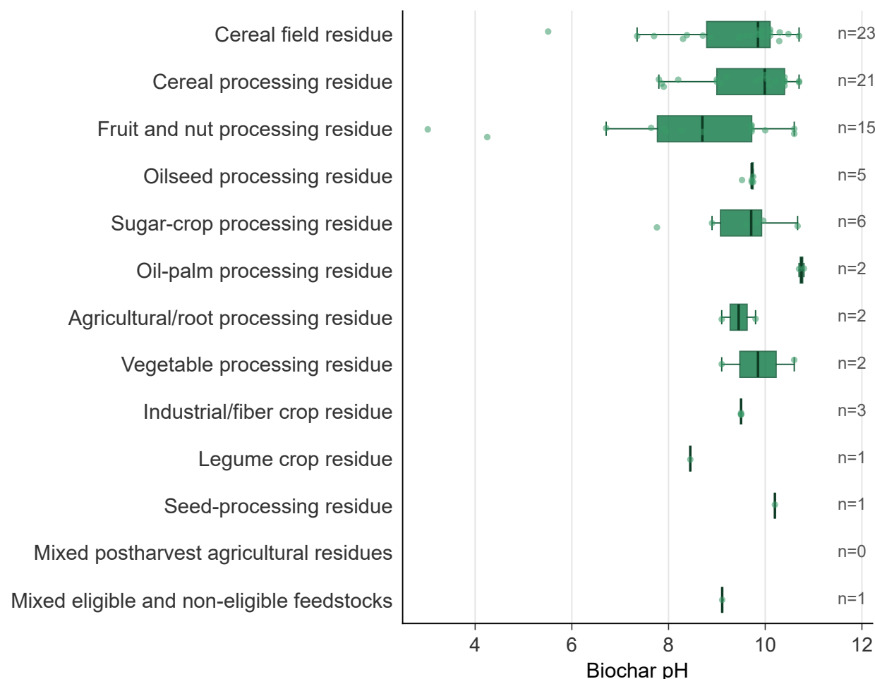
A Biochar pH (n = 82 treatments)
