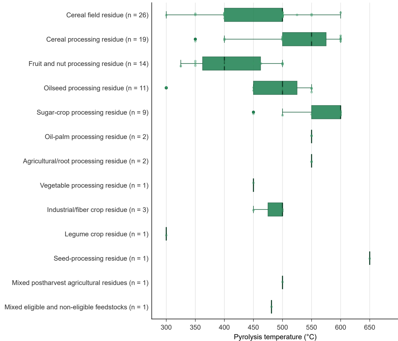
Temperature by feedstock category (n = 91 treatments)
