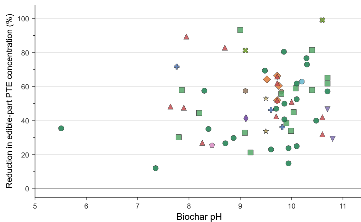
A Biochar pH (n = 67 treatments)
