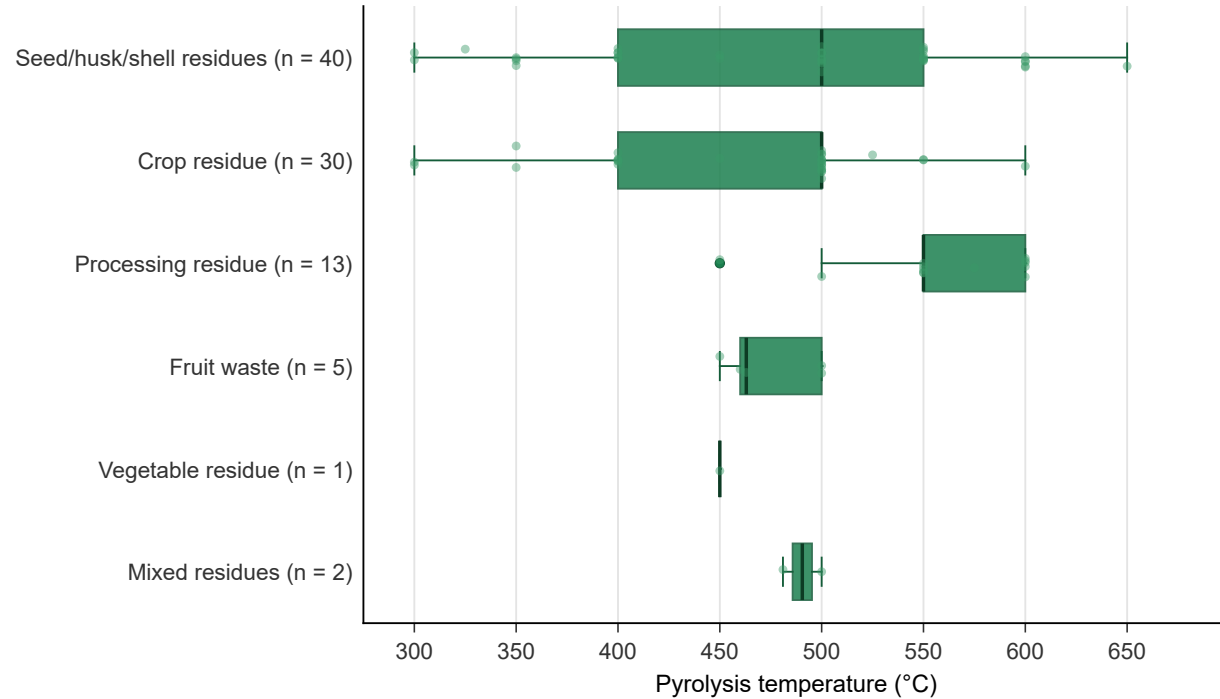
B Temperature by feedstock category (n = 91 treatments)
