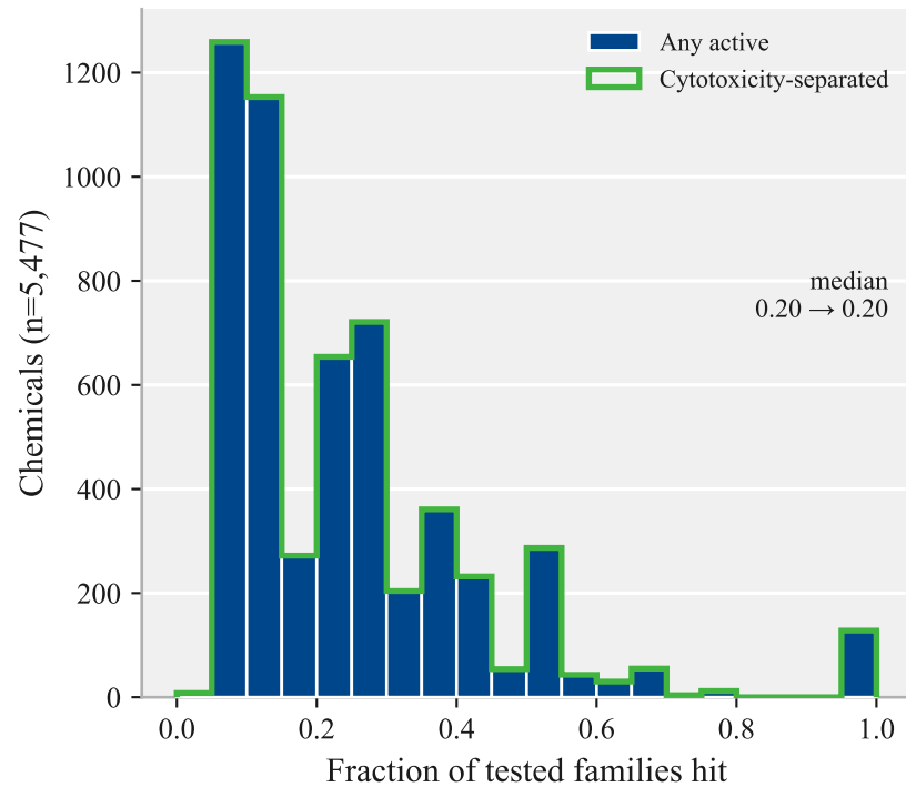
(B) Default bound: filter is inert
