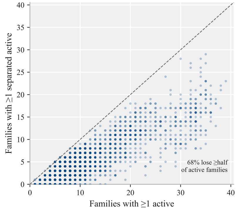
(C) Raw family counts, estimated bound
