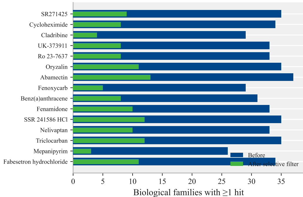
(B) Largest family collapses
