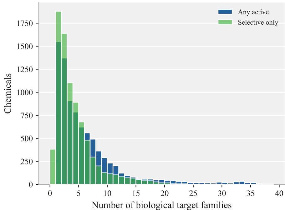
(A) Promiscuity before vs after filter
