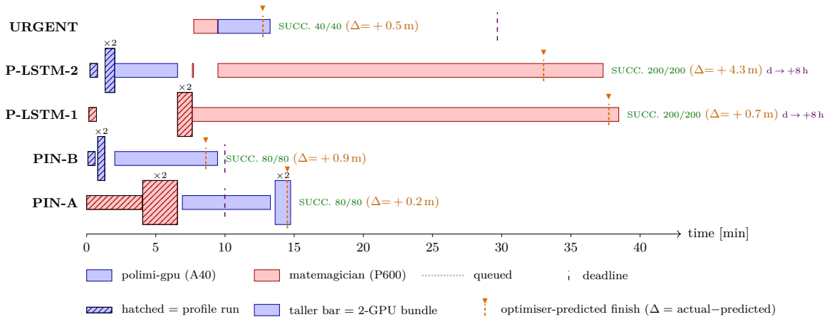
Figure 4.2: Scenario 2 timeline (run 2026-06-25, t=0 at first dispatch). The cluster is full when URGENT arrives, so the plan preempts a single prio-1 lstm-small (P-LSTM-2): IJM stops it and places URGENT on P600×1, then migrates URGENT onto A40×1 the moment PIN-B ends, where it meets its deadline; the evicted patient resumes on P600 — the gap-then-resume visible on its row. Predicted-finish overlay as in Fig. 4.1: most jobs land within \sim 1 min, the outlier being P-LSTM-2 at +4.3 min — preempted and then resumed sharing matemagician , its final run hit co-location contention ( \sim 10.6 s/epoch vs. the solo profile’s \sim 9.2 s) a solo profile cannot foresee. Which preemptible bundle the plan picks is the proxy’s choice (Appendix A).
