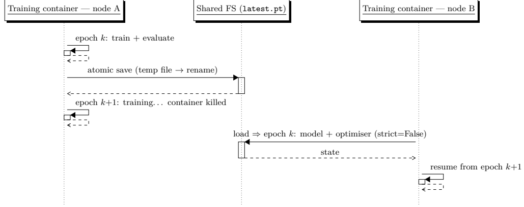
Figure 2.7: Stop and resume across nodes. Each lifeline is the training container (the trainer process the worker launched via docker run ) on its node. The container checkpoints after each epoch with a temp-file-and-rename, so latest.pt is never half-written; a stop kills it mid-epoch, and the next run — here on a different node, possibly a different torch version — loads latest.pt and continues, so only the interrupted epoch k+1 is recomputed.
