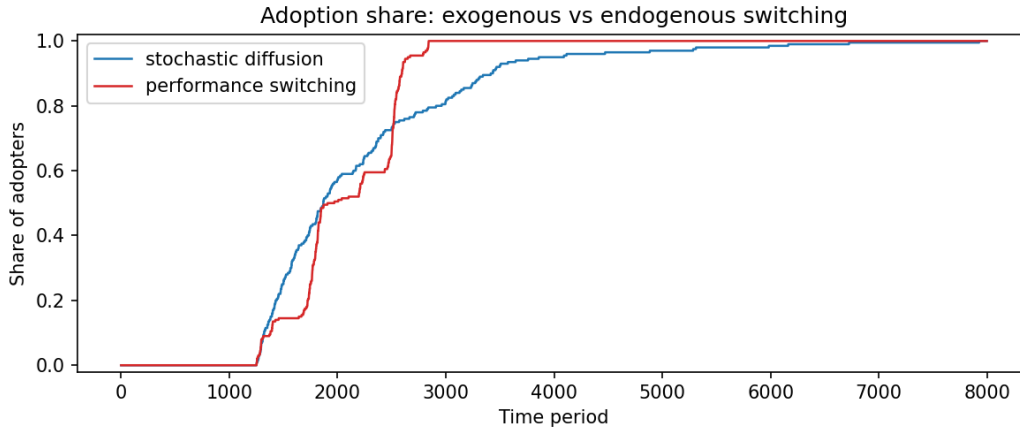
Figure 12: Adoption share over time for exogenous stochastic diffusion ( \pi = 10^{-3} ) and endogenous CE-based switching on paired shocks (seed 71). The endogenous share is steplike, creeping while the switching score is negative and bursting when it turns positive, and reaches full adoption by period 2842; the diffusion share ramps smoothly and crosses 0.99 only at period 6164.
