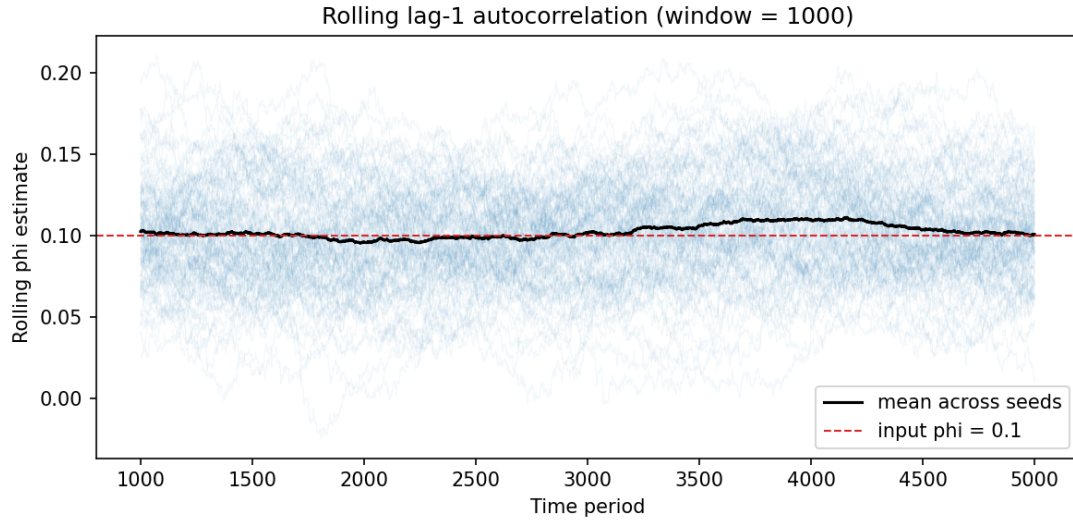
Figure 8: Rolling lag-1 autocorrelation of returns under the null rule, on a 1000-period sliding window for each of 100 seeds (faint lines); the black line is the cross-seed mean, the dashed line the input \phi = 0.10 . The mean trace stays flat for the full run, total range 0.016 over the 4001 periods with a complete window: no drift in the effective AR coefficient in the absence of adoption.
