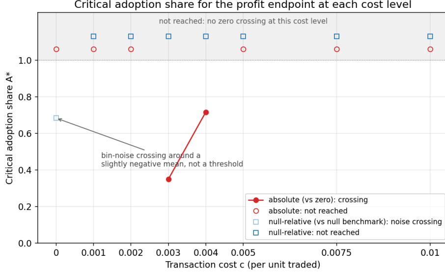
Figure 7: Per-cost critical adoption shares A^*_{\text{profit}} across the full cost grid. Filled red circles mark A^*_{\text{profit,abs}} , the smallest binned share at which mean absolute net profit crosses zero from below, defined at c = 0.003 ( A^* = 0.35 ) and c = 0.004 ( A^* = 0.72 ) only. Open markers in the shaded band above A^* = 1 mark cost levels whose curve produces no zero crossing: absolute net profit is positive at every observed share for c \leq 0.002 and negative at every observed share for c \geq 0.005 , and the null-relative curve crosses nowhere at any positive cost. The de-emphasised, annotated open square at c = 0 ( A \approx 0.68 ) is the null-relative bin-noise crossing around a slightly negative mean discussed in the text, not a threshold reading.
