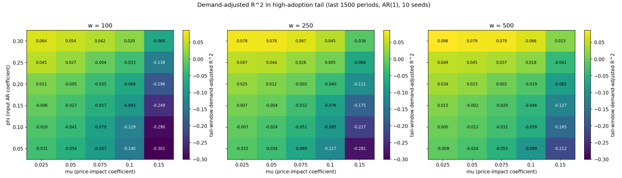
Figure 15: Mean demand-adjusted R^2 over the same high-adoption tail, same layout: the tail-depth view behind section 6.5. The reading falls with \mu in every \phi row, from positive values up to 0.06 to 0.09 at low \mu and high \phi down to -0.21 to -0.30 at (\phi = 0.05, \mu = 0.15) depending on the window: at the strongest price impact the independent signal is pushed below zero, not merely halved.
