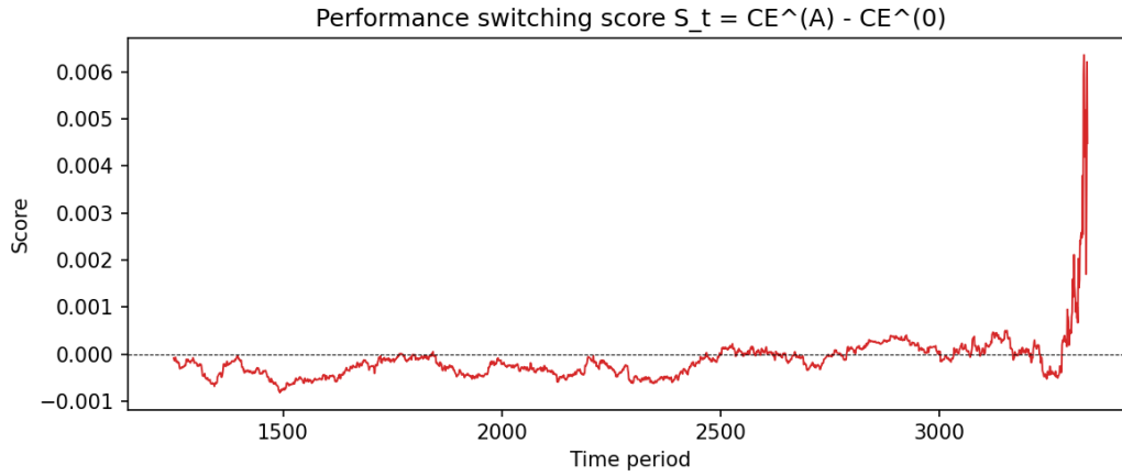
Figure 13: The switching score S_t = CE_t^{(A)} - CE_t^{(0)} driving the endogenous run of Figure 12, shown from the adoption release at period 1250 until shortly after full adoption. The score hovers slightly below zero through most of the run-up, negative in 88 percent of pre-saturation periods, and the sharp spike to about +0.0064 arrives only after full adoption, once adopter trading has amplified the persistence the rule feeds on.
