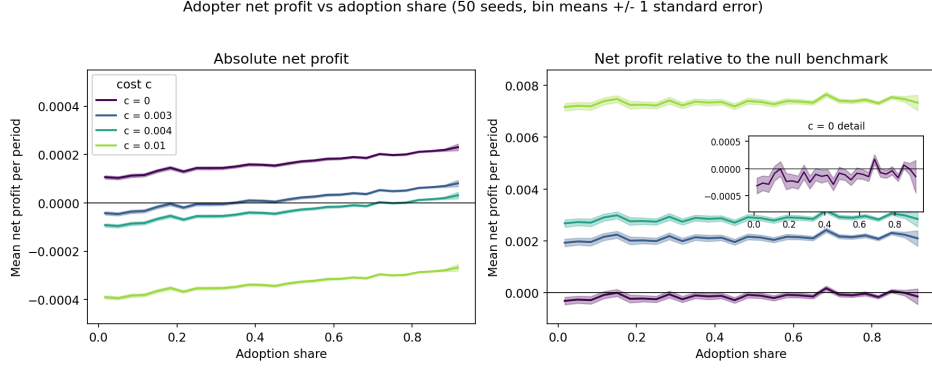
Figure 6: Per-period adopter net profit versus adoption share at four representative cost levels: c = 0 , the two crossing levels c = 0.003 and 0.004 , and the largest cost on the grid, c = 0.01 . Net profit is pooled over 50 paired-shock seeds into 30 adoption-share bins; lines are bin means, bands \pm 1 standard error, and bins with 10 or fewer observations are dropped, ending the curves short of full adoption. Left: absolute net profit q_t^{(A)} r_{t+1} - c |q_t^{(A)}| ; every curve rises with adoption, rising cost shifts the curves down in parallel, and only the c = 0.003 and c = 0.004 curves cross zero. Right: net profit relative to the null benchmark, on a vertical scale roughly an order of magnitude larger set by the null’s cost bill; the positive-cost curves sit uniformly above zero, ordered by cost level, while the c = 0 curve sits slightly below zero at almost every observed share (inset detail).
