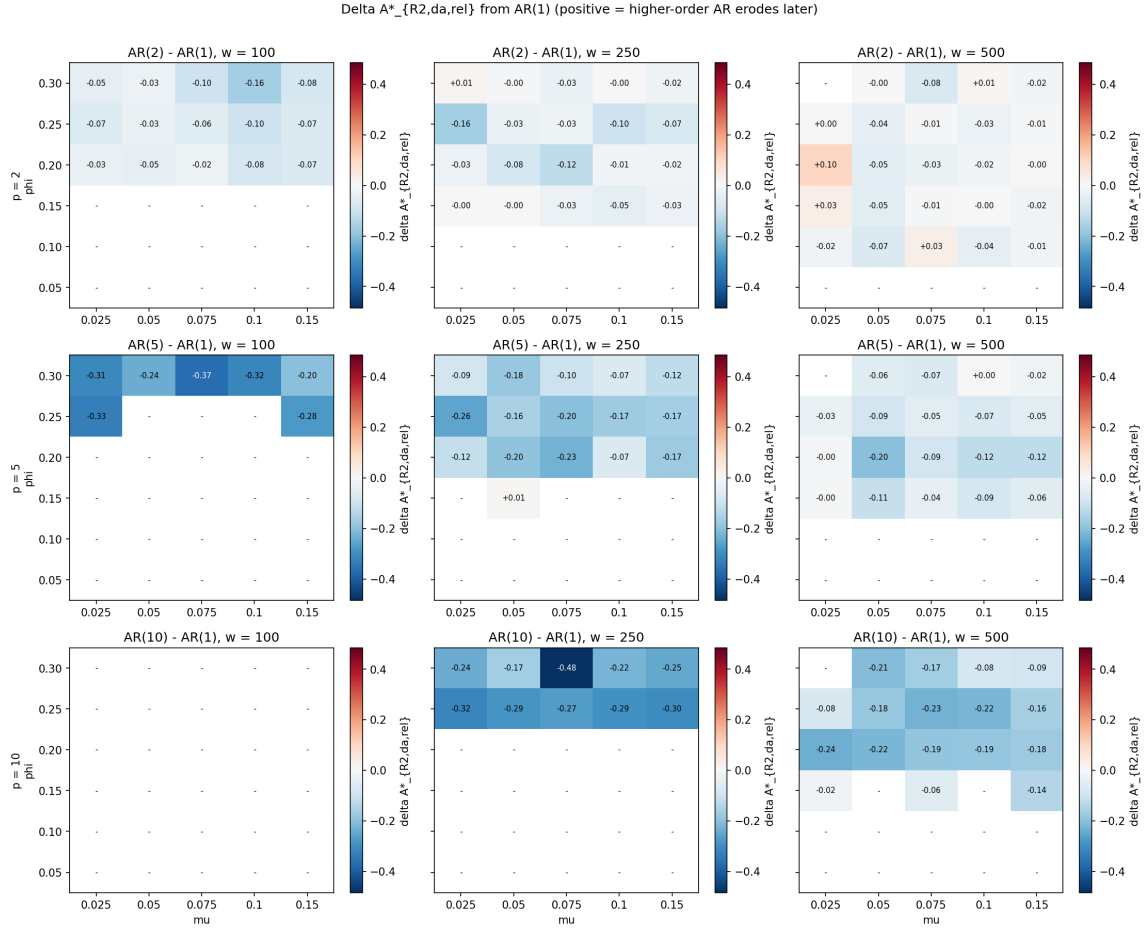
Figure 18: Cell-by-cell difference in the demand-adjusted threshold, A^*_{R2,da,rel} at order p minus its AR(1) value, for p \in \{2, 5, 10\} (rows) and w \in \{100, 250, 500\} (columns); dashes mark cells where either side is undefined. The populated cells are predominantly mildly negative, with mean deltas of -0.04 , -0.14 , and -0.20 for p = 2, 5, 10 : higher-order rules cross somewhat earlier, having less signal to lose, and nowhere does the mechanism reverse.
