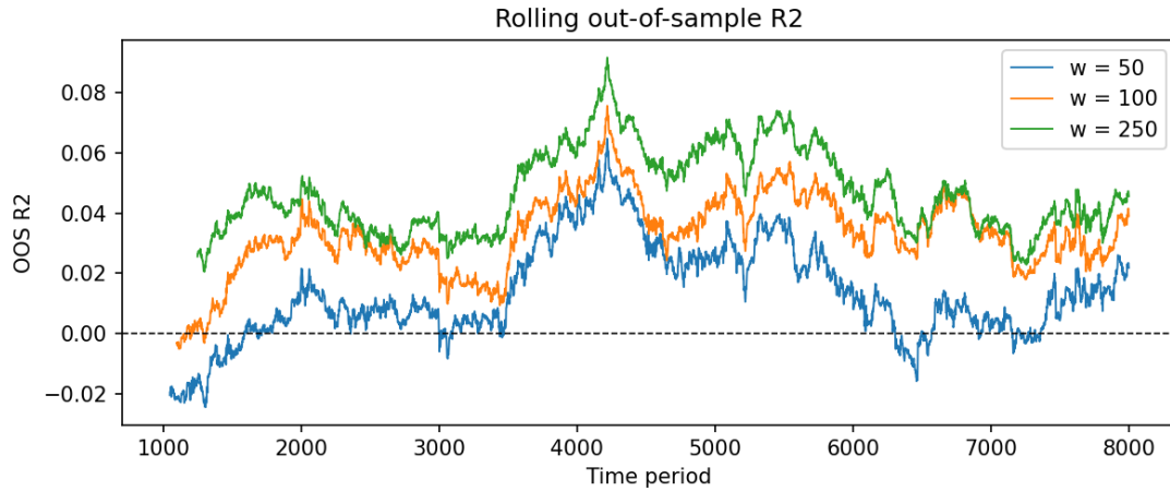
Figure 9: Rolling out-of-sample R^2 of the one-step AR(1) forecast against realised returns, on a trailing 1000-period window, for estimation windows w = 50, 100 , and 250 on the same null-market path (input \phi = 0.25 , seed 43); the dashed line marks zero. The traces co-move because they score one path; longer windows sit almost everywhere higher ( w = 100 and w = 250 briefly cross around periods 6800 to 6900), w = 250 stays positive at every evaluated period, and w = 50 intermittently dips below zero.
