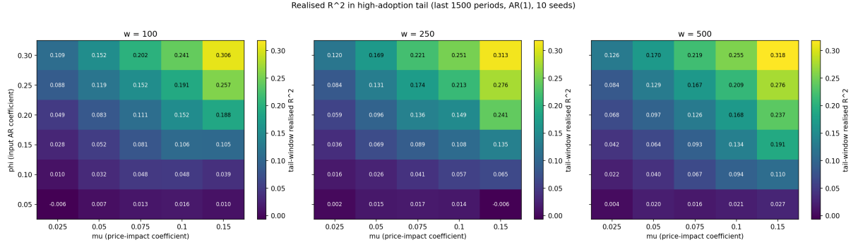
Figure 14: Mean realised-return R^2 over the high-adoption tail (final 1500 periods) across the (\mu, \phi) grid for the AR(1) rule, one panel per window w , 10 seeds per cell. The tail reading rises with both \phi and \mu in every panel, peaking at 0.31 to 0.32 in the top-right corner, while the \phi = 0.05 row stays near zero: the self-fulfilment channel at grid scale and the realised-channel non-result of section 7.3.
