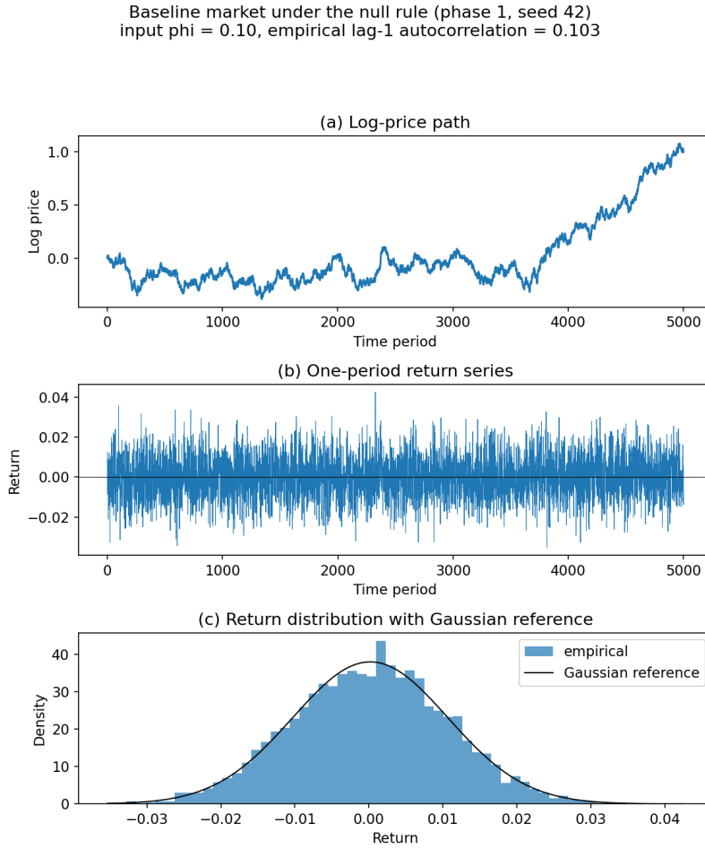
Figure 1: Baseline market under the null rule (phase 1: N = 200 , T = 5000 , \mu = 0.05 , input \varphi = 0.10 , seed 42). (a) The log-price path wanders with no systematic drift. (b) The one-period return series is roughly stationary around zero. (c) The return histogram is symmetric and close to the Gaussian reference density built from the empirical mean and standard deviation. The empirical lag-1 autocorrelation of returns is 0.103, against the input 0.10.
