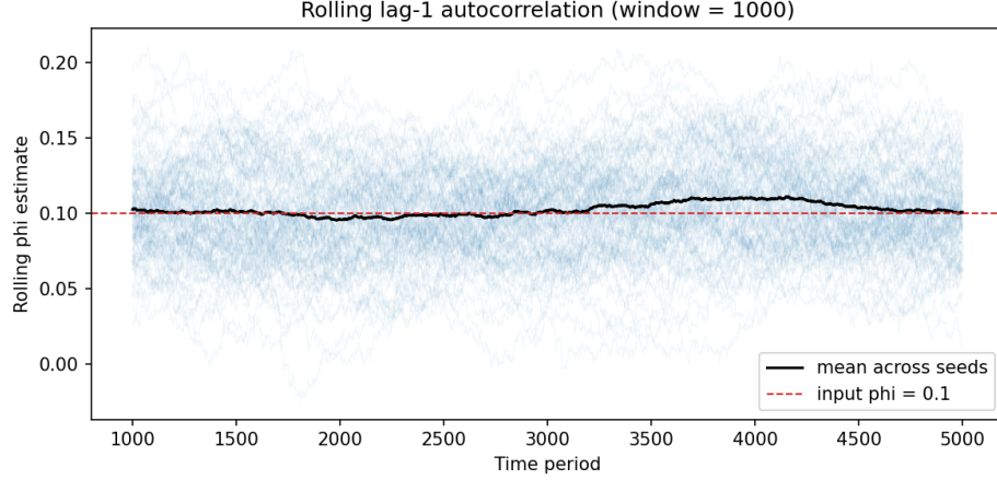
Figure 1: Rolling lag-1 autocorrelation of returns under the null rule, estimated on a 1000-period sliding window for each of 100 seeds (faint lines). The black line is the cross-seed mean and the dashed line marks the input \phi = 0.10 . The mean trace stays flat for the full run, with a total range of 0.016 over the 4001 periods where the window is complete, so the effective AR coefficient shows no drift in the absence of adoption.
