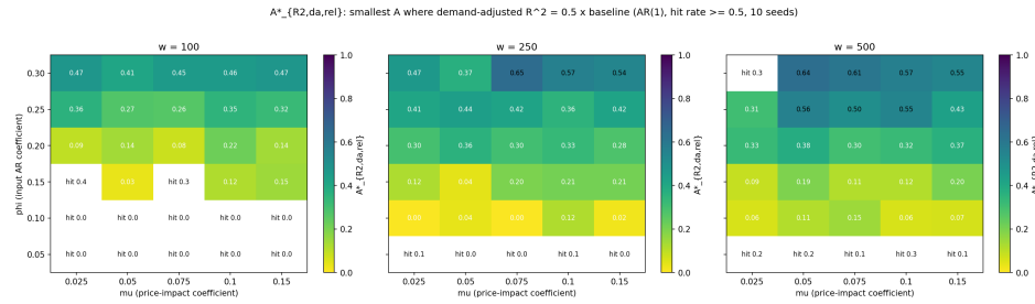
Figure 6: Relative demand-adjusted threshold A^*_{R^2, da, rel} across the (\mu, \phi) grid for the AR(1) rule, one panel per forecast window w \in \{100, 250, 500\} . Each cell shows the smallest adoption share at which the rolling demand-adjusted R^2 fell to half its low-adoption baseline, averaged over the crossing seeds; cells where fewer than half of the 10 seeds crossed print their hit rate instead (for example “hit 0.3”) and are left blank. The crossing share rises with the input \phi , from very low values in the \phi = 0.10 row, where the baseline is itself near zero, to 0.37 to 0.65 at \phi = 0.30 , and is roughly flat across \mu ; the \phi = 0.05 row is unreachable in every panel.
