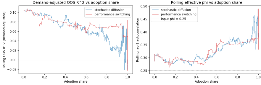
Figure 4: Rolling out-of-sample R^2 against the demand-adjusted return (left) and rolling lag-1 autocorrelation of realised returns (right) versus adoption share, for exogenous stochastic diffusion ( \pi = 10^{-3} ) and endogenous CE-based switching on paired shocks (seed 71), trailing 1000-period windows. The regimes share the pre-adoption segment (demand-adjusted R^2 near 0.104, effective coefficient 0.286 to 0.314 at zero adoption, against the input \phi = 0.25 marked by the dashed line), then decline (left) and rise (right) along overlapping paths, converging at full adoption. The switching curve sits above the stochastic one on the left at intermediate shares because the endogenous run sweeps those shares in few periods relative to the metric window; the vertical segments at share 1.0 collect each run’s post-saturation stretch.
