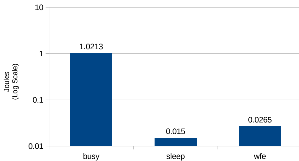
Altra HWMon single core Average Energy Consumption for busy, sleep and wfe binaries (Ten, five second runs of each)
