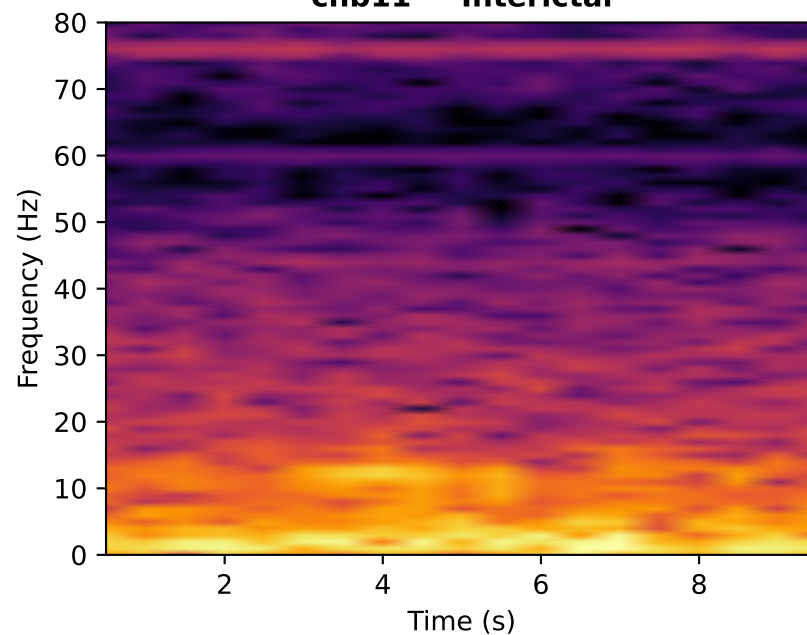
chb11 — Interictal
