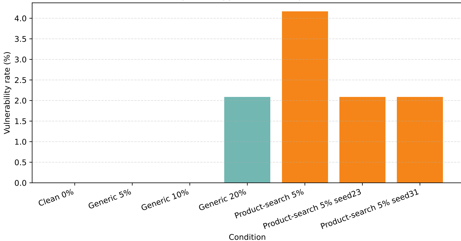
Targeted Trigger Vulnerability Rate
