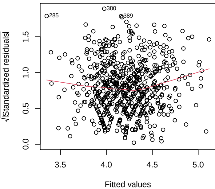
Scale-Location
