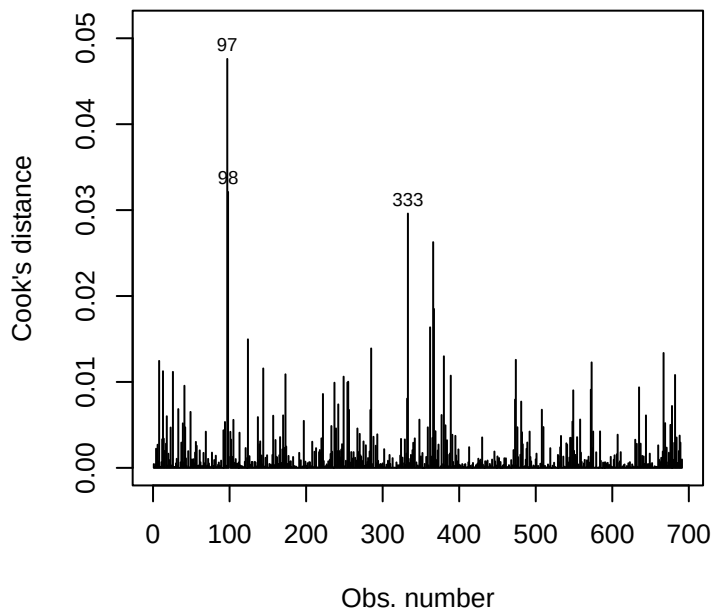
Cook's distance
