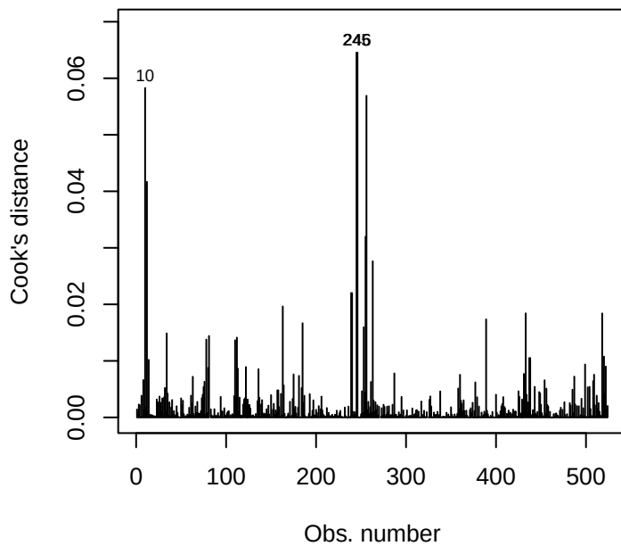
Cook's distance
