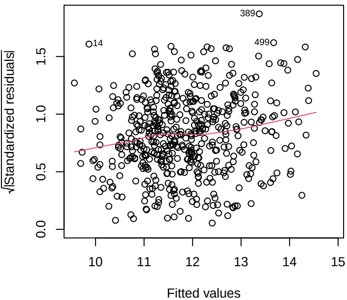
Scale-Location
