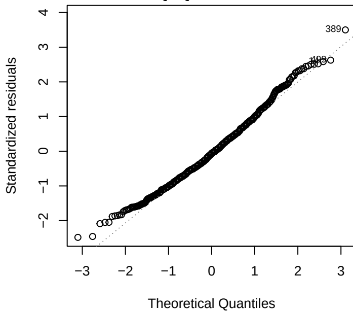
Q-Q Residuals
