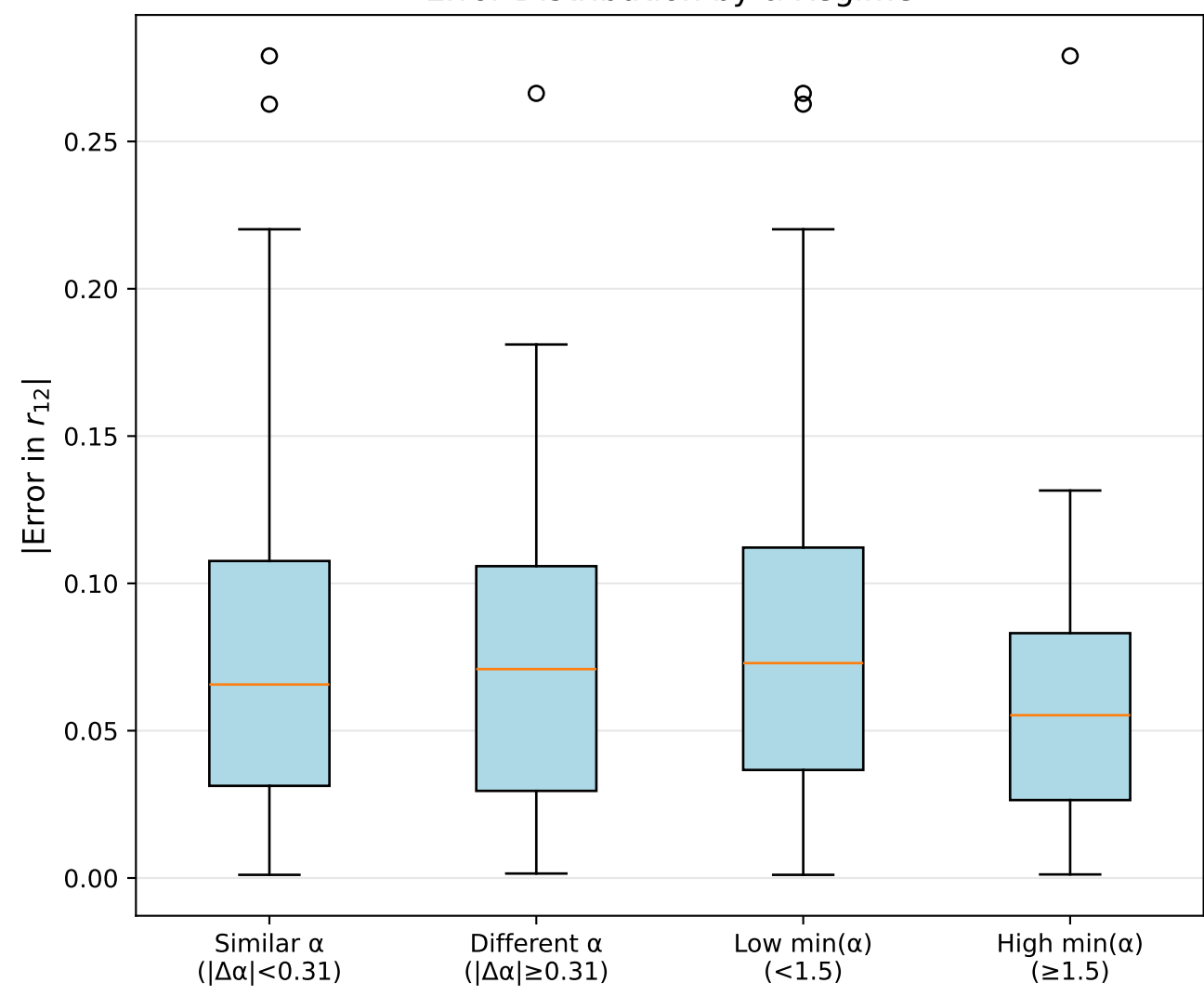
Error Distribution by \alpha Regime
