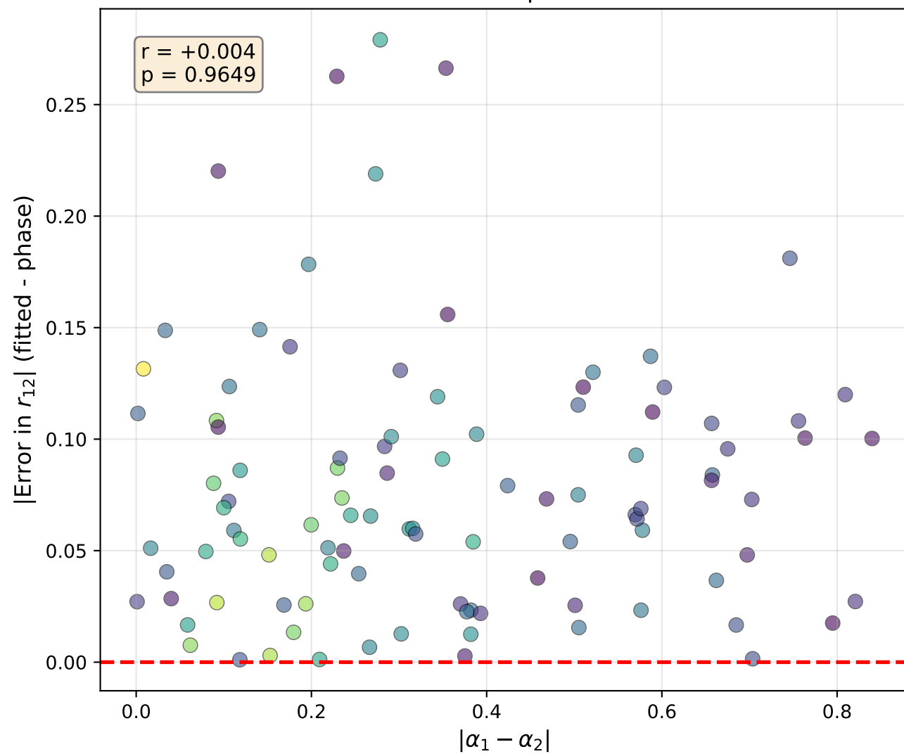
Exponent Pairs: Colored by |Error|
