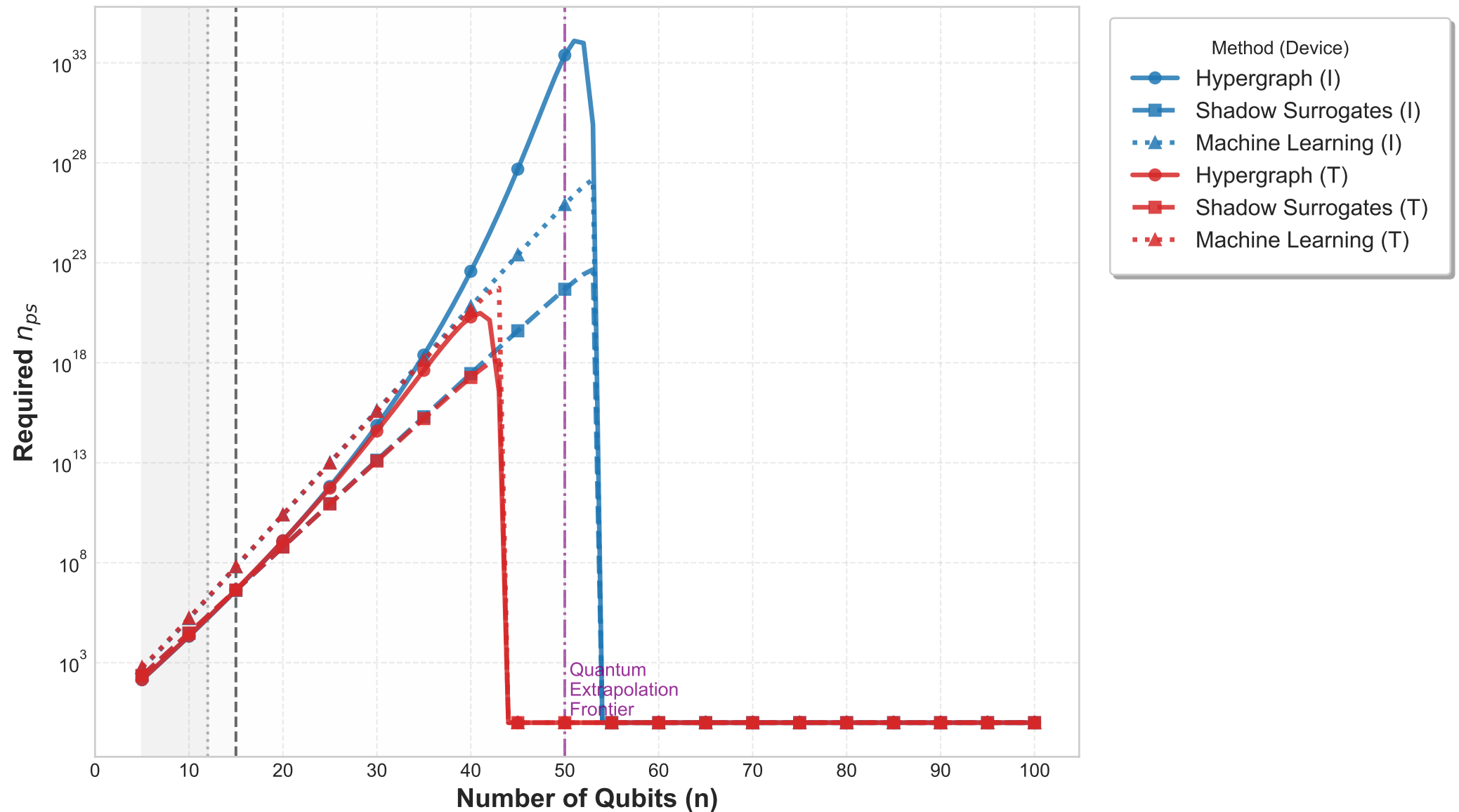
Relaxation Noise ( \gamma=0.1 | Readout: 1% | \eta=0.01 )
