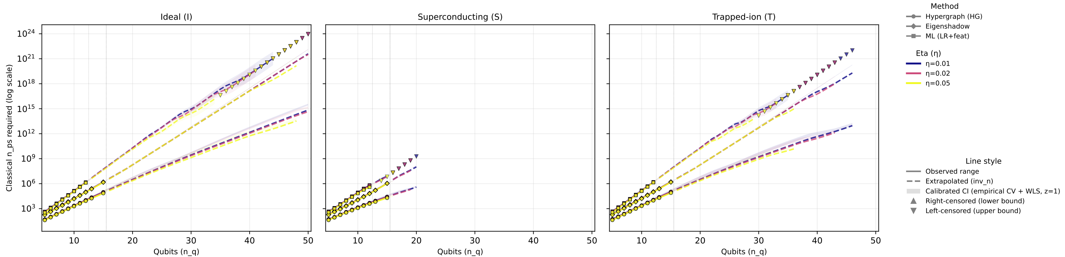
Unified Comparison (1x3 devices) — channel=Dephasing, p=0.01 , readout=1%
