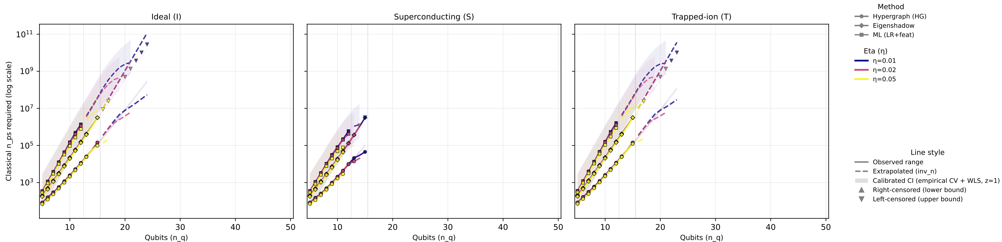
Unified Comparison (1x3 devices) — channel=Dephasing, p=0.05 , readout=0%
