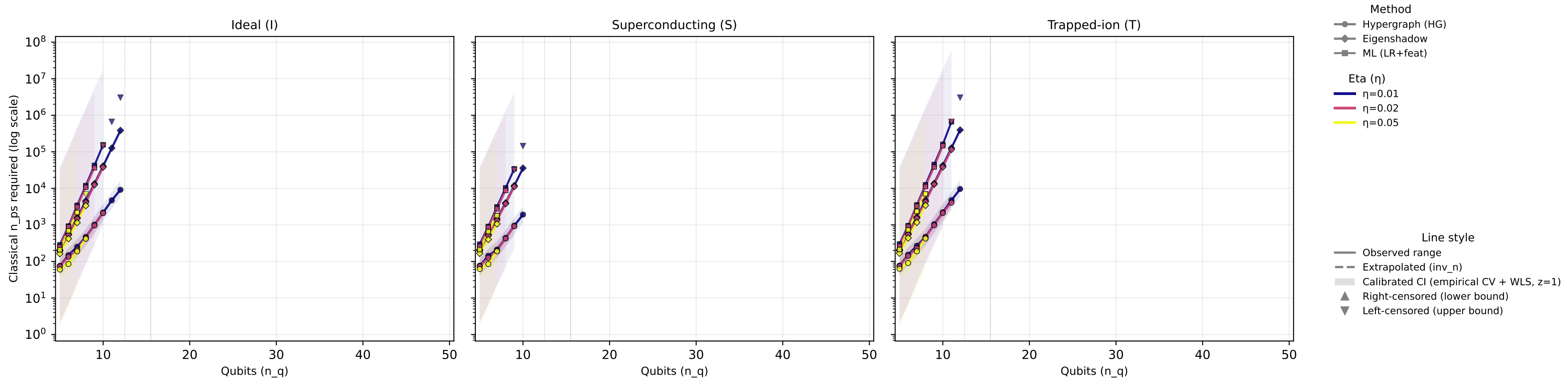
Unified Comparison (1x3 devices) — channel=Dephasing, p=0.1, readout=0%
