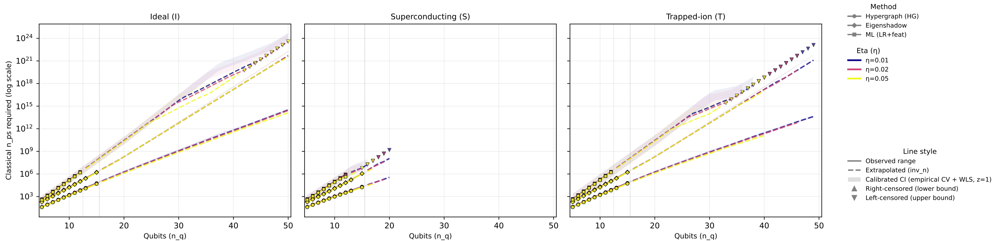
Unified Comparison (1x3 devices) — channel=Depolarizing, p=0.01 , readout=1%
