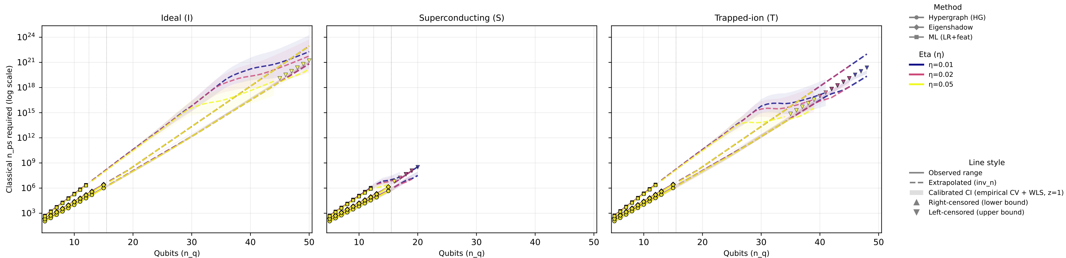
Unified Comparison (1x3 devices) — channel=Relaxation, p=0.05, readout=0%
