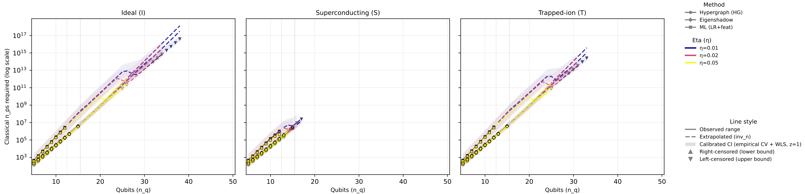
Unified Comparison (1x3 devices) — channel=Relaxation, p=0.1, readout=1%
