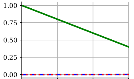
Depolarizing
