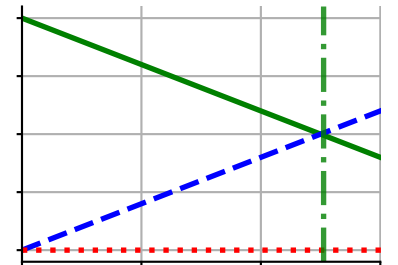
Dephasing
