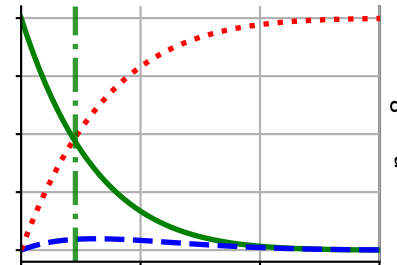
Thermal Relaxation
