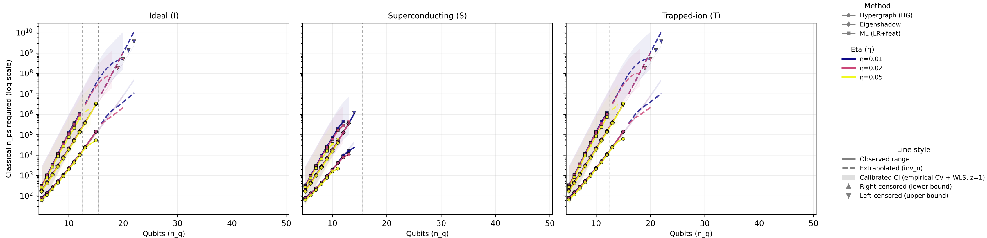
Unified Comparison (1x3 devices) — channel=Dephasing, p=0.05 , readout=1%
