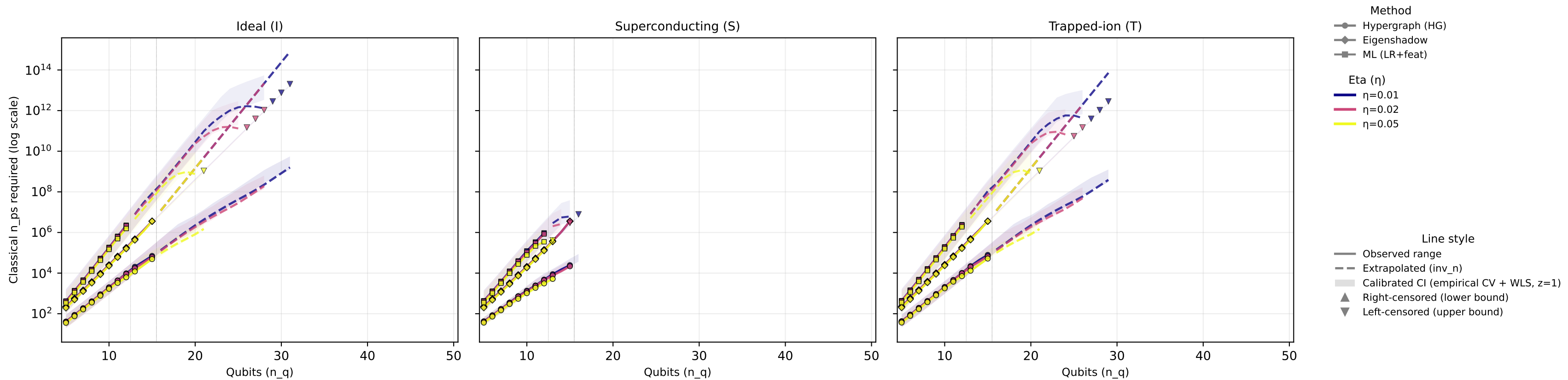
Unified Comparison (1x3 devices) — channel=Depolarizing, p=0.05, readout=1%
