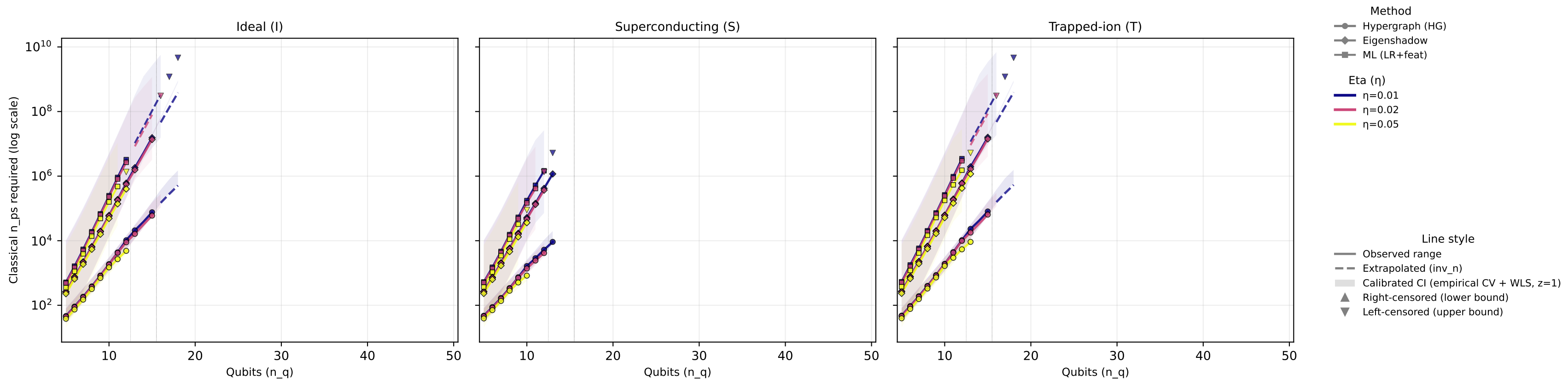
Unified Comparison (1x3 devices) — channel=Depolarizing, p=0.1 , readout=0%
