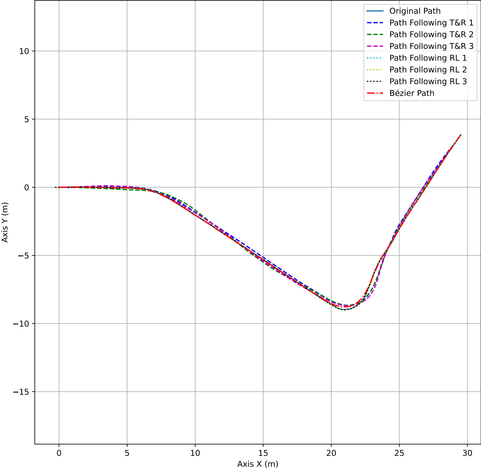
Corridor Path Comparison
