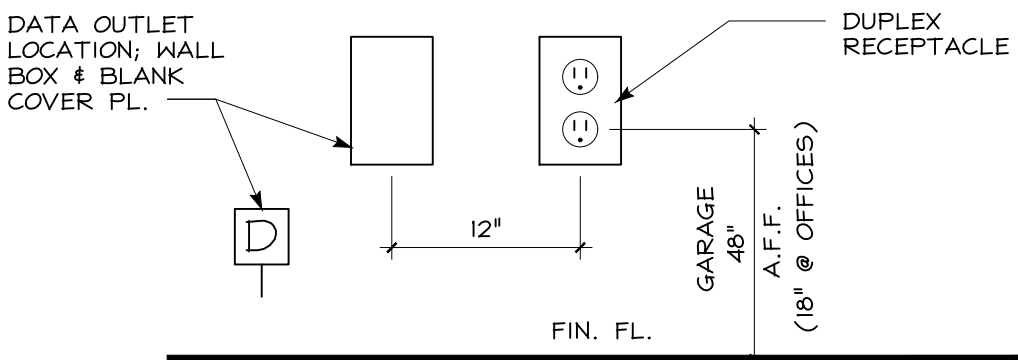
OUTLET MOUNTING DETAIL NO SCALE
