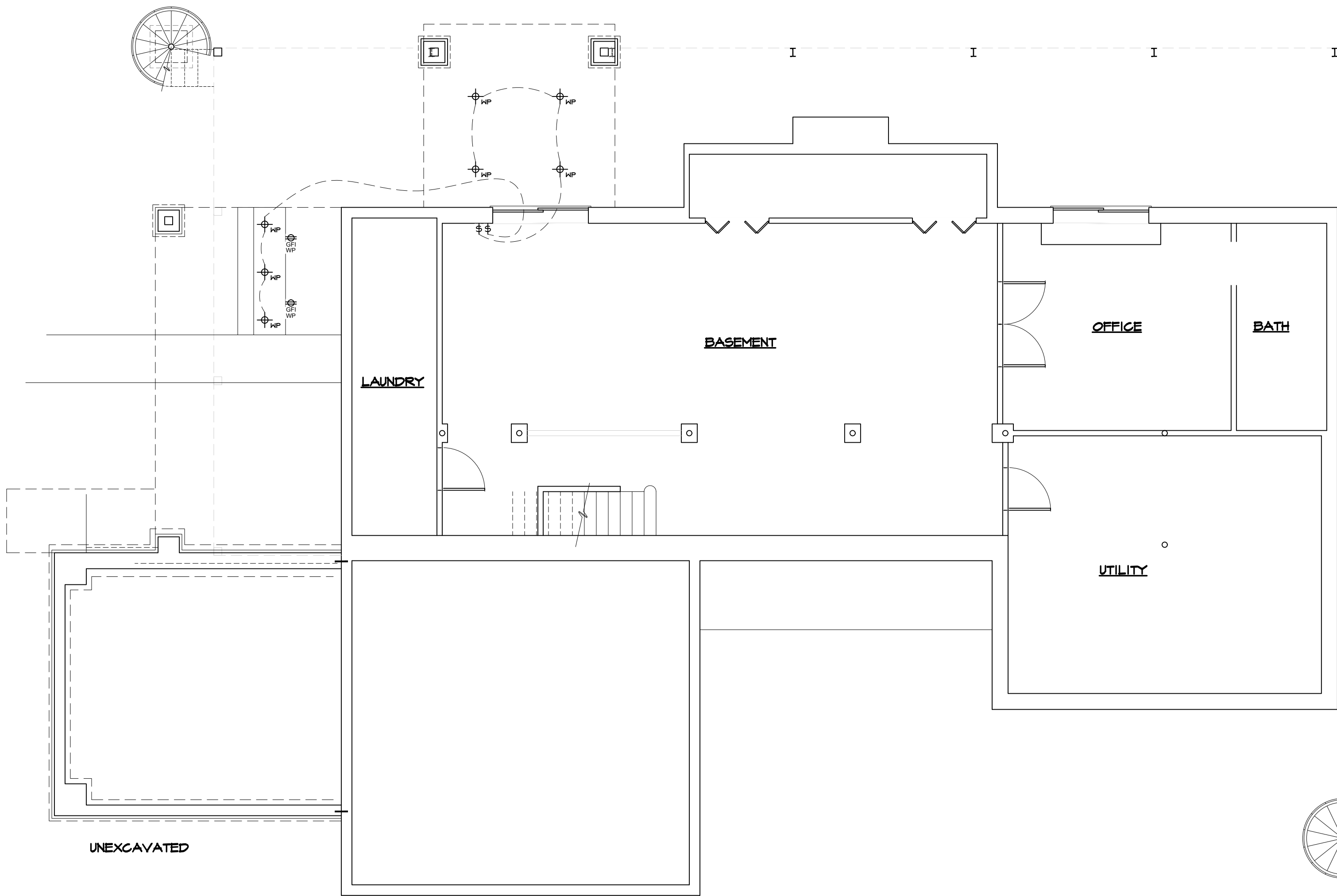
BASEMENT ELECTRICAL PLAN SCALE: 1/4" = 1'-0"
