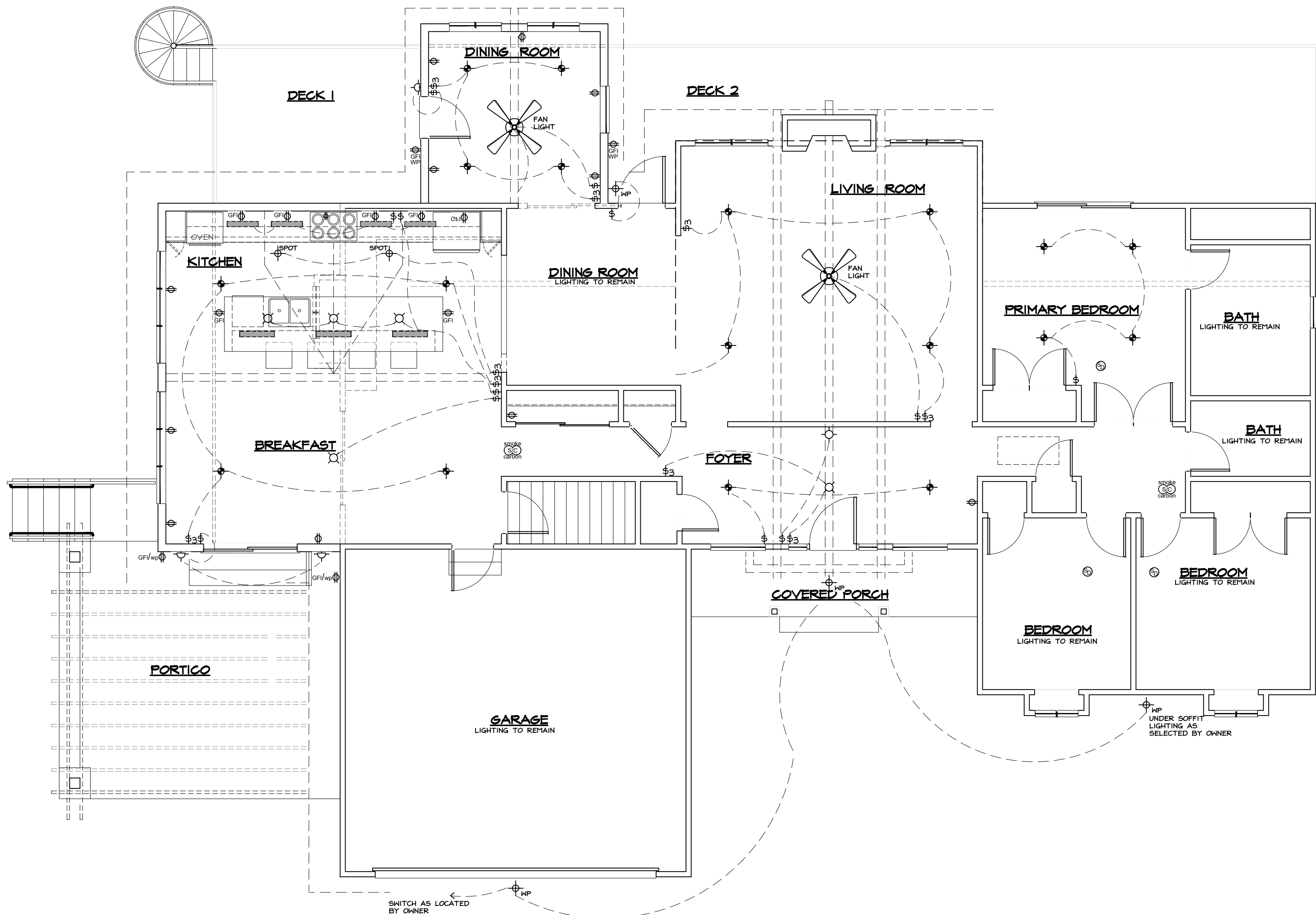
FIRST FLOOR ELECTRICAL PLAN SCALE: 1/4" = 1'-0"
