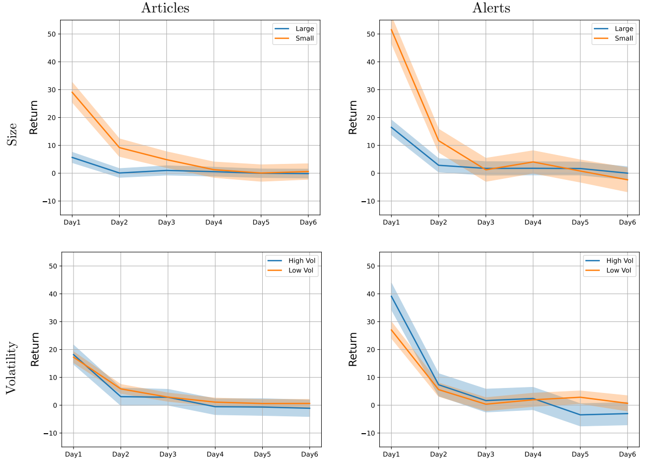
Figure 7: Heterogeneous News Assimilation: Size and Volatility
