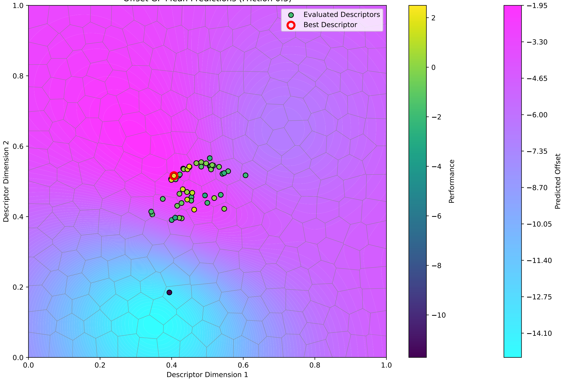
Offset GP Mean Predictions (Friction 0.3)
